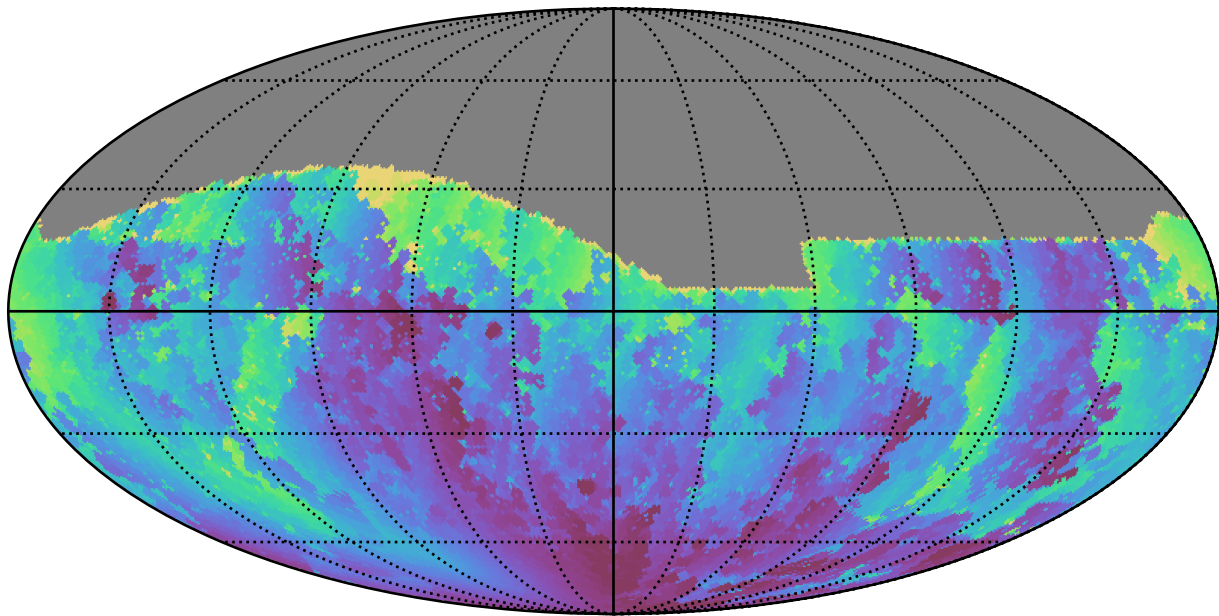
noroll_mjdp0_v3.4_10yrs All sky g band: Min solarElong
