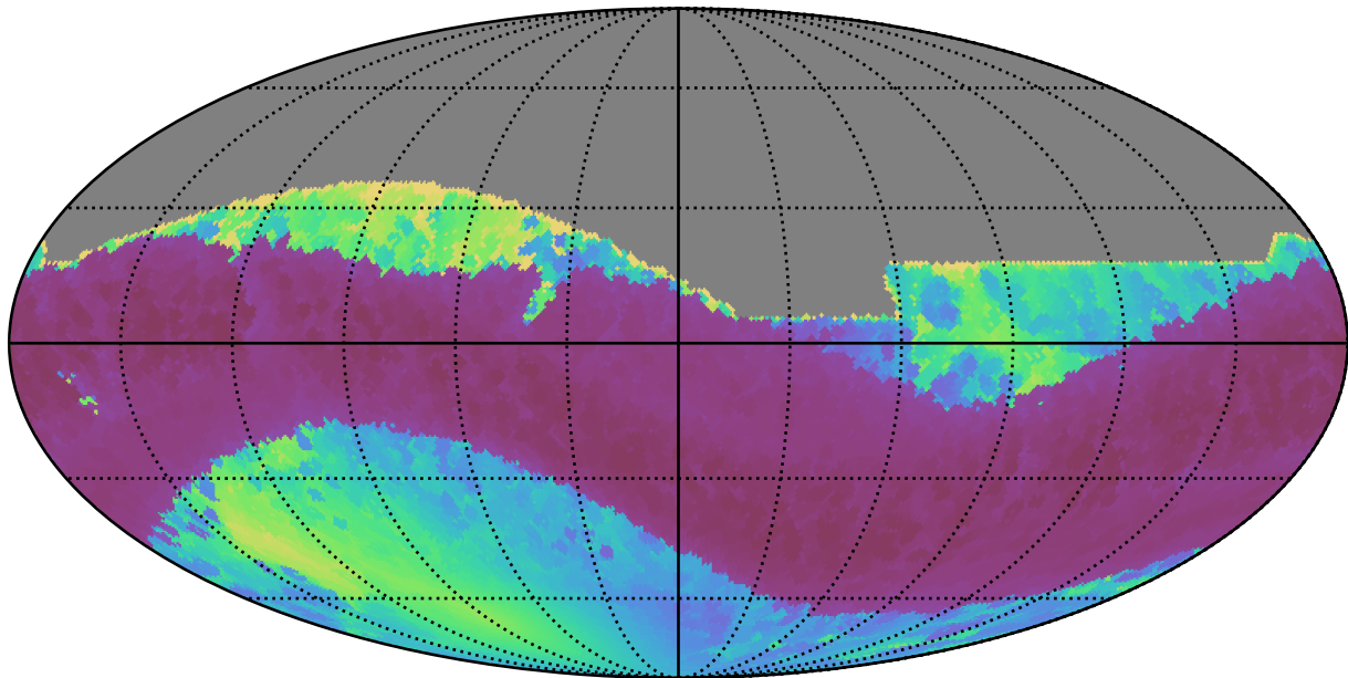
noroll_mjdp0_v3.4_10yrs All sky all bands: Min solarElong
