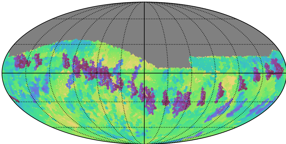
noroll_mjdp0_v3.4_10yrs Yr 1 z band: Min skyBrightness
