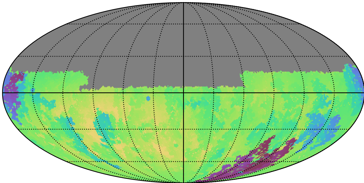
noroll_mjdp0_v3.4_10yrs Yr 1 u band: Min skyBrightness
