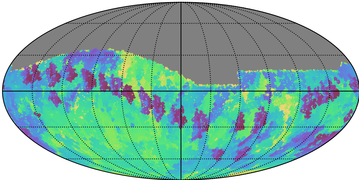
noroll_mjdp0_v3.4_10yrs Yr 1 i band: Min skyBrightness
