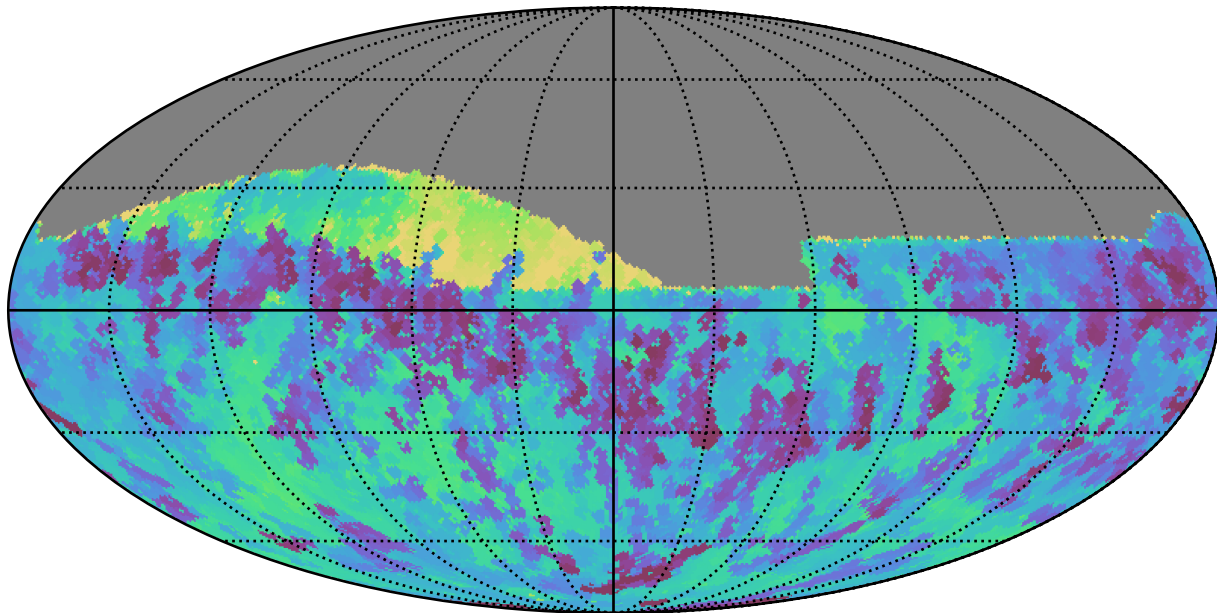
noroll_mjdp0_v3.4_10yrs Yr 1 all bands: Min skyBrightness
