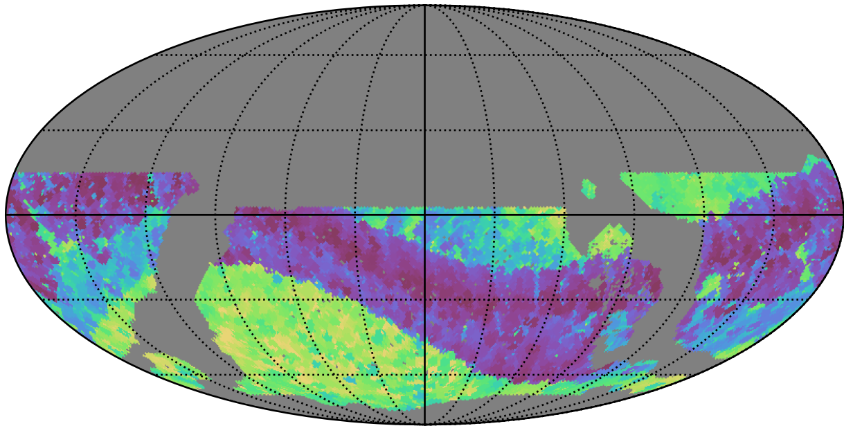
noroll_mjdp0_v3.4_10yrs WFD z band: Min skyBrightness
