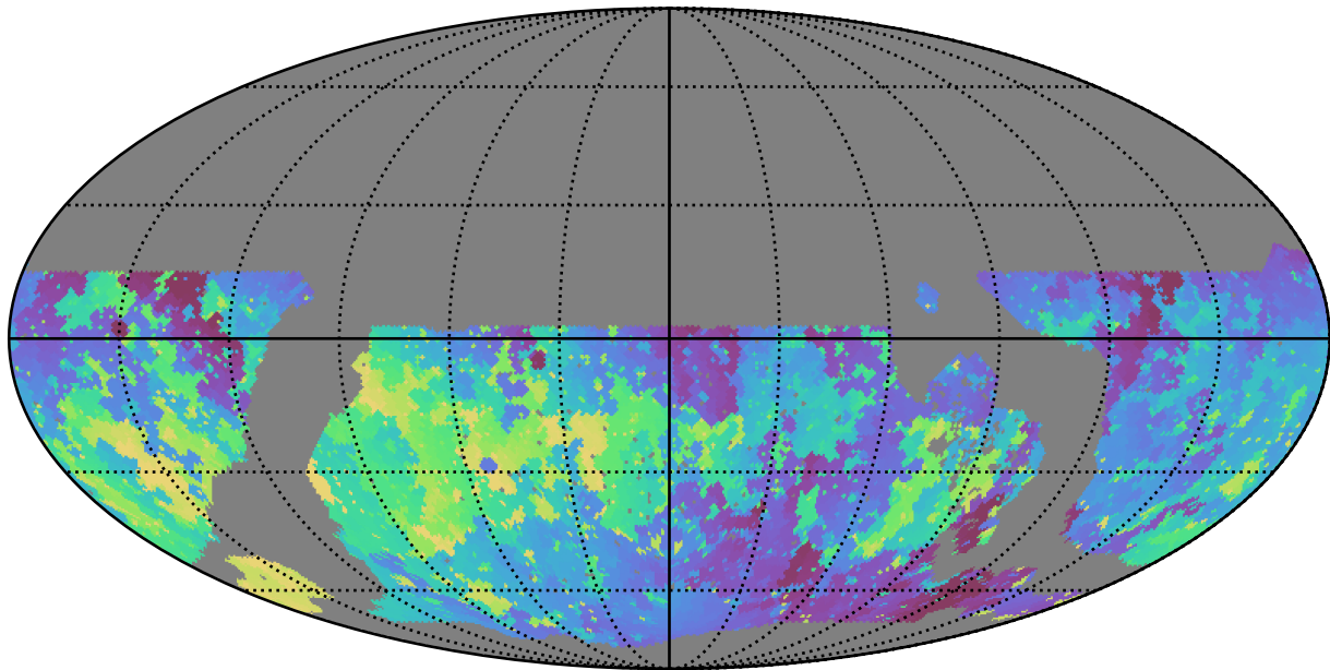
noroll_mjdp0_v3.4_10yrs WFD u band: Min skyBrightness
