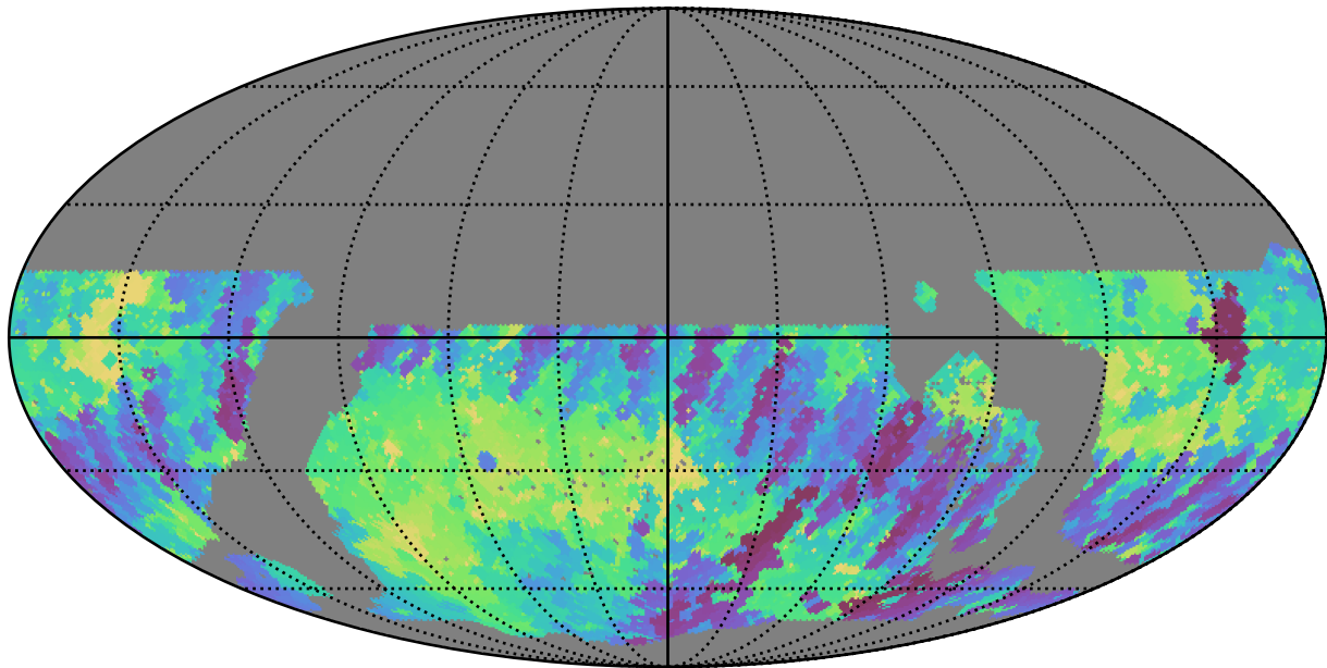
noroll_mjdp0_v3.4_10yrs WFD r band: Min skyBrightness
