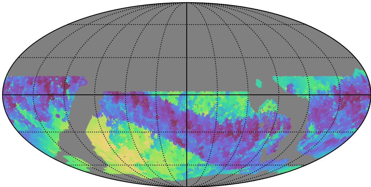
noroll_mjdp0_v3.4_10yrs WFD i band: Min skyBrightness
