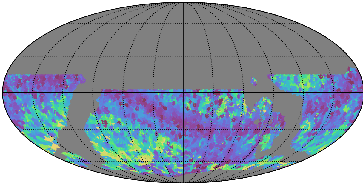
noroll_mjdp0_v3.4_10yrs WFD all bands: Min skyBrightness
