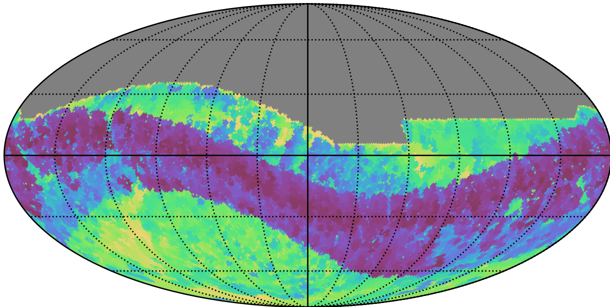
noroll_mjdp0_v3.4_10yrs All sky z band: Min skyBrightness
