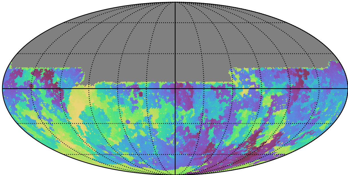
noroll_mjdp0_v3.4_10yrs All sky u band: Min skyBrightness
