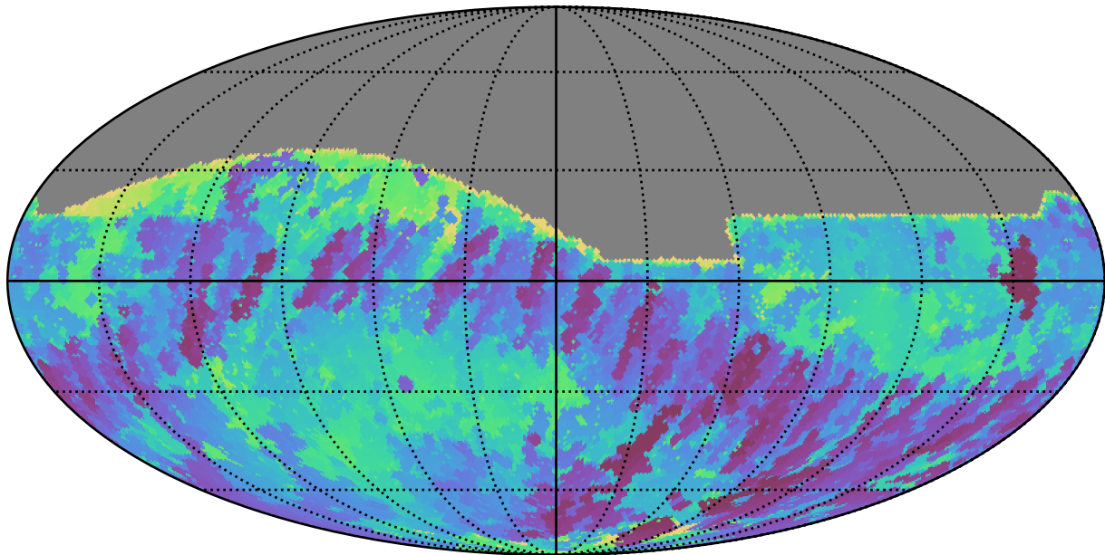
noroll_mjdp0_v3.4_10yrs All sky r band: Min skyBrightness
