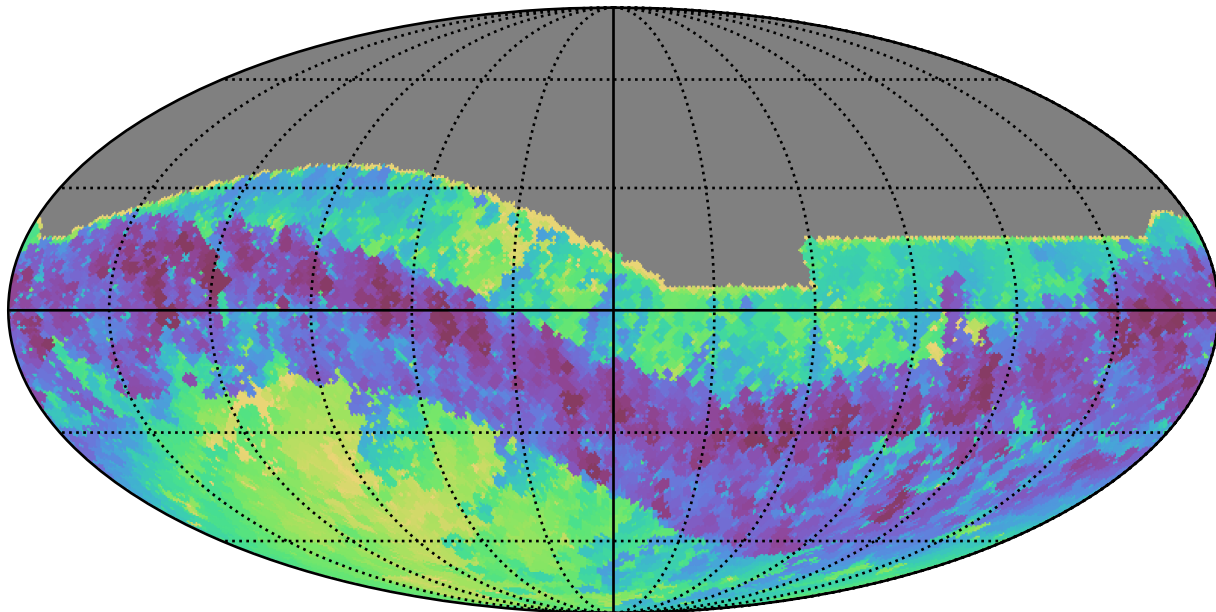
noroll_mjdp0_v3.4_10yrs All sky i band: Min skyBrightness
