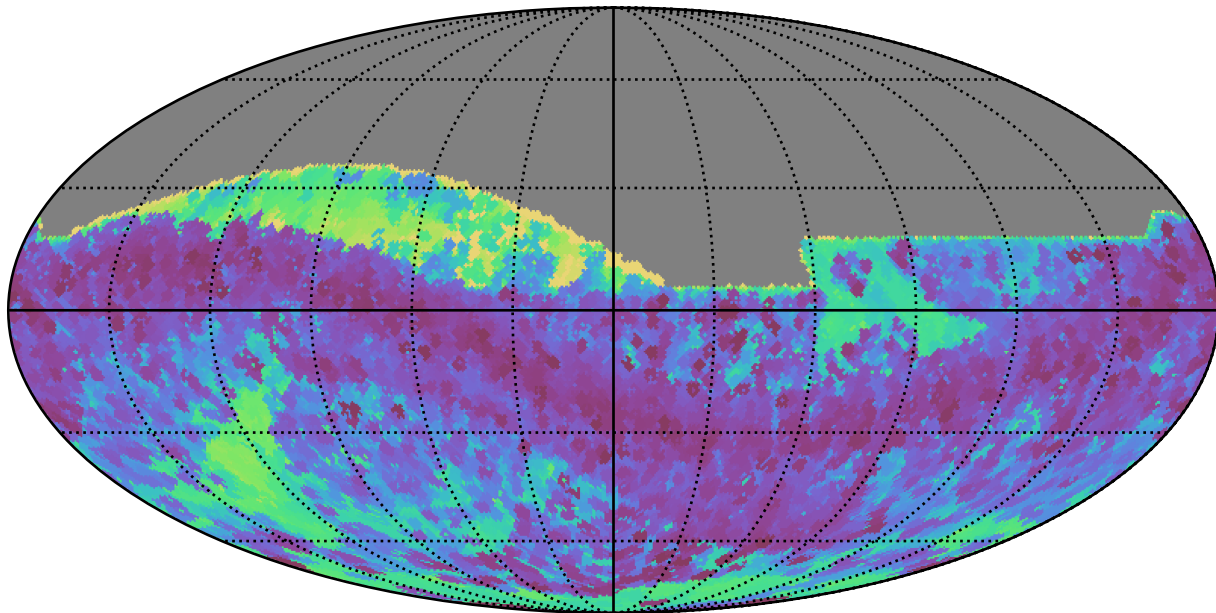
noroll_mjdp0_v3.4_10yrs All sky all bands: Min skyBrightness
