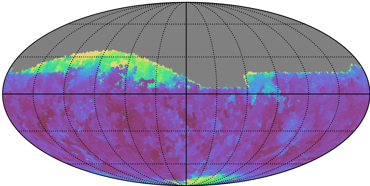
noroll_mjdp0_v3.4_10yrs Yr 1 r band: Min seeingGeom
