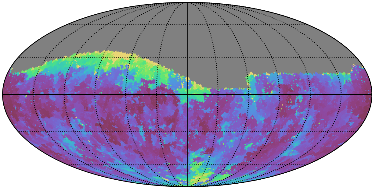
noroll_mjdp0_v3.4_10yrs Yr 1 g band: Min seeingGeom
