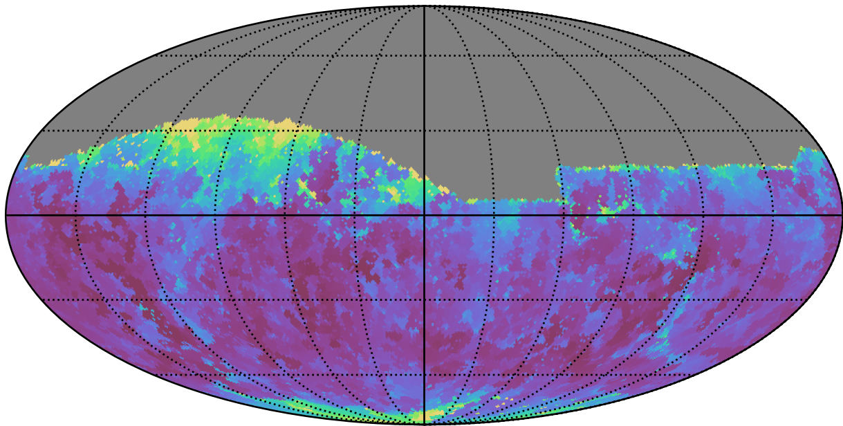
noroll_mjdp0_v3.4_10yrs Yr 1 z band: Min seeingEff
