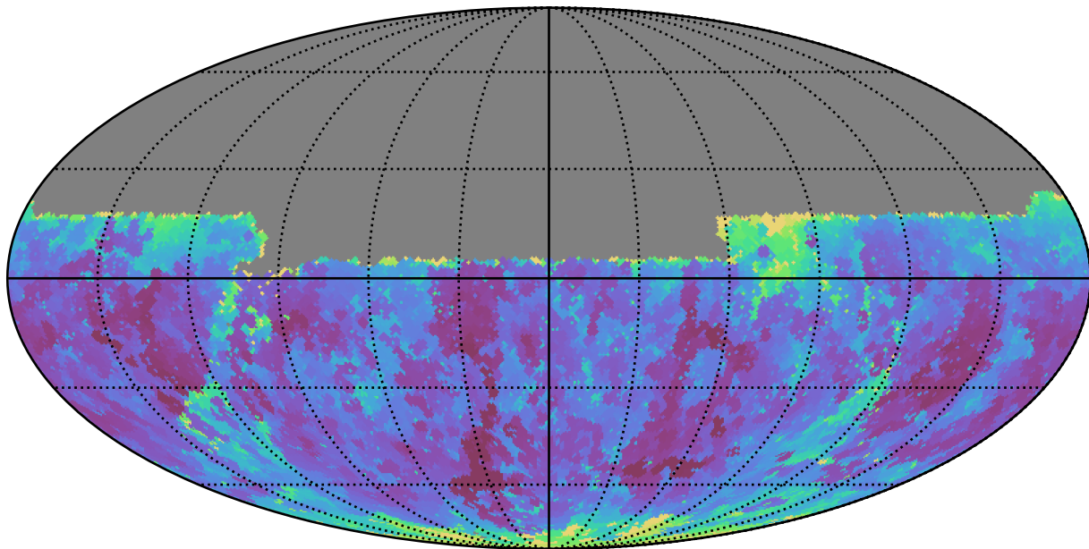
noroll_mjdp0_v3.4_10yrs Yr 1 y band: Min seeingEff
