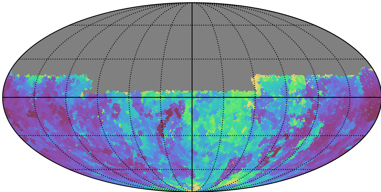
noroll_mjdp0_v3.4_10yrs Yr 1 u band: Min seeingEff
