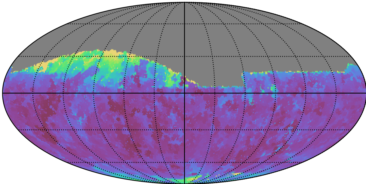
noroll_mjdp0_v3.4_10yrs Yr 1 i band: Min seeingEff
