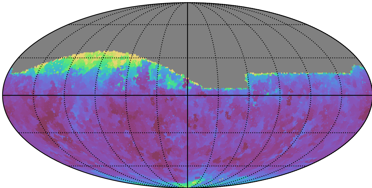
noroll_mjdp0_v3.4_10yrs Yr 1 all bands: Min seeingEff
