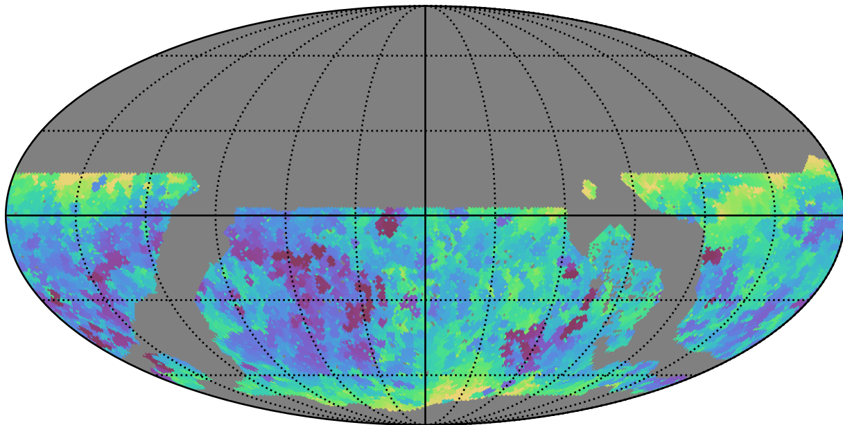
noroll_mjdp0_v3.4_10yrs WFD i band: Min seeingEff
