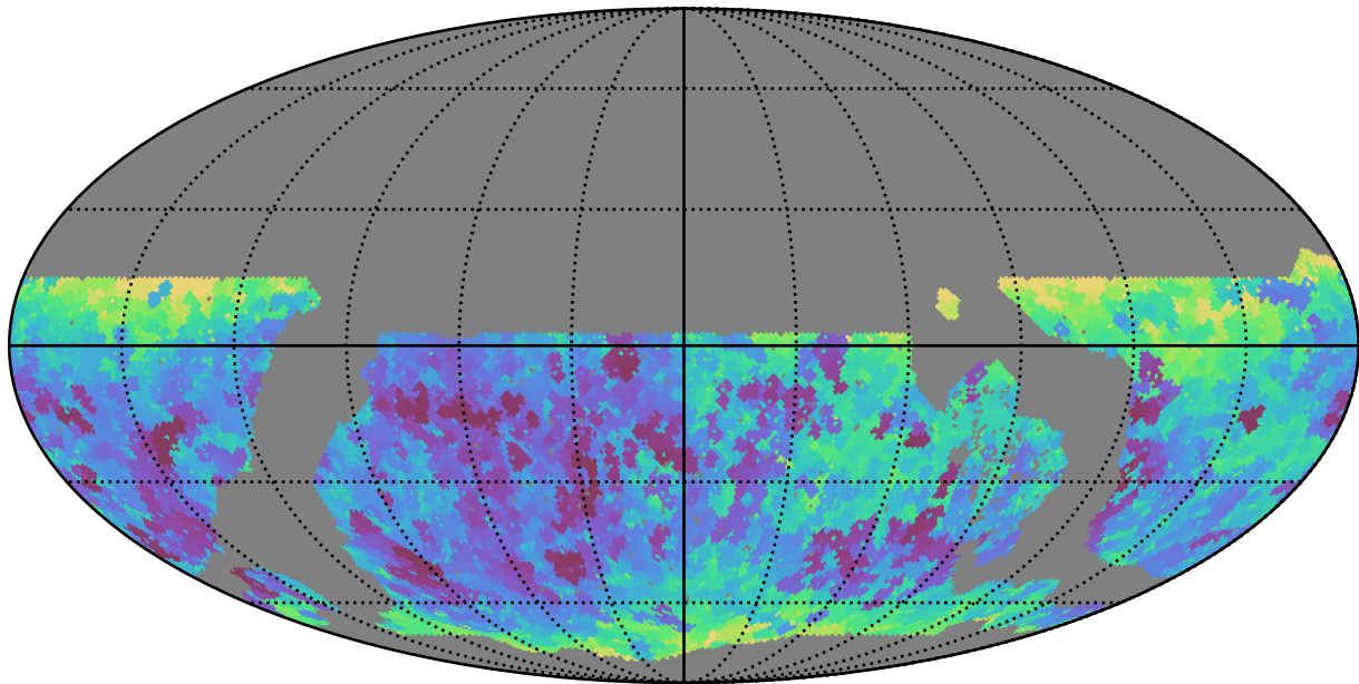
noroll_mjdp0_v3.4_10yrs WFD all bands: Min seeingEff
