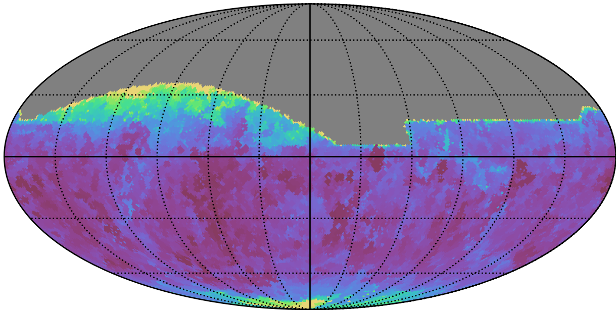
noroll_mjdp0_v3.4_10yrs All sky z band: Min seeingEff
