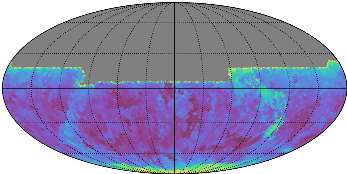
noroll_mjdp0_v3.4_10yrs All sky y band: Min seeingEff
