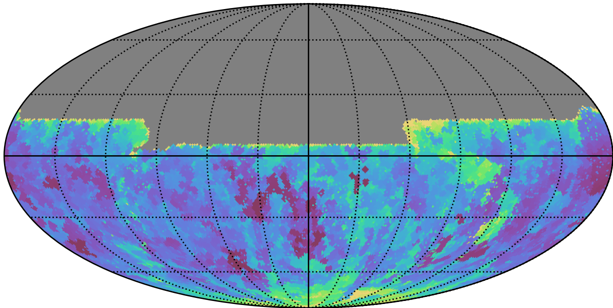
noroll_mjdp0_v3.4_10yrs All sky u band: Min seeingEff
