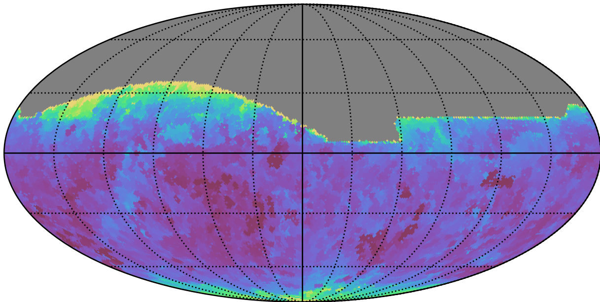
noroll_mjdp0_v3.4_10yrs All sky i band: Min seeingEff
