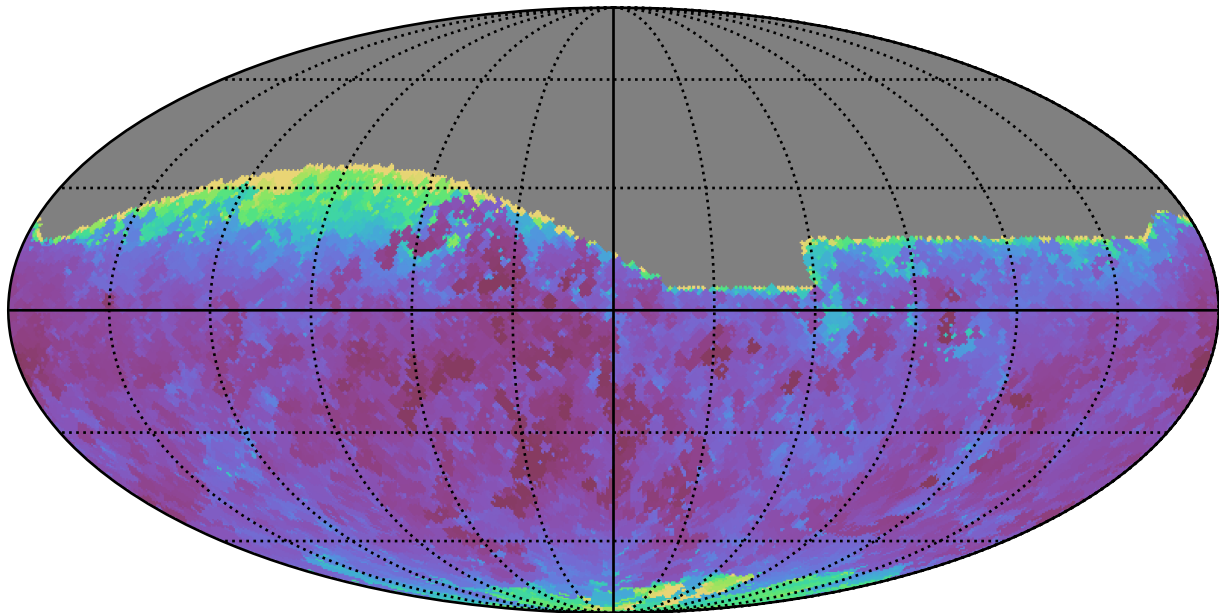
noroll_mjdp0_v3.4_10yrs All sky g band: Min seeingEff
