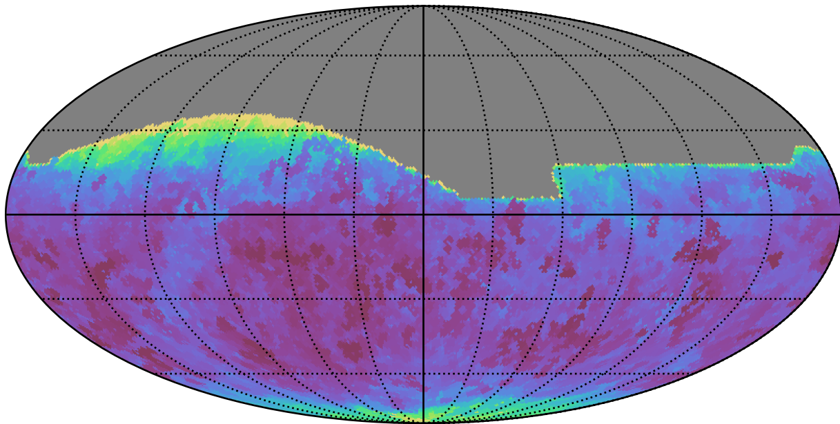
noroll_mjdp0_v3.4_10yrs All sky all bands: Min seeingEff
