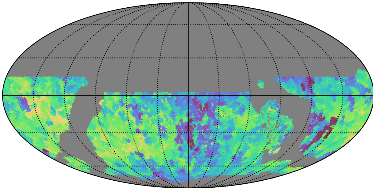
noroll_mjdp0_v3.4_10yrs WFD all bands: Min saturation_mag
