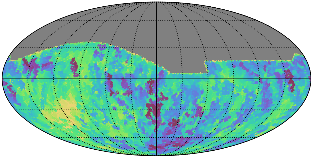
noroll_mjdp0_v3.4_10yrs All sky z band: Min saturation_mag
