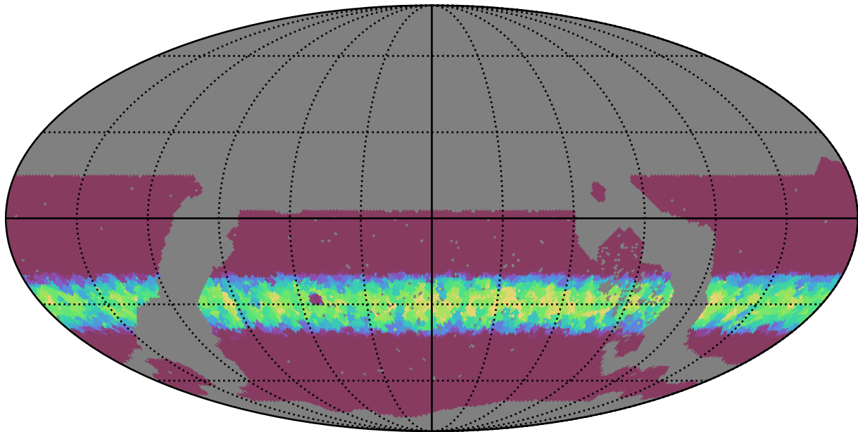
noroll_mjdp0_v3.4_10yrs WFD r band: Min normairmass
