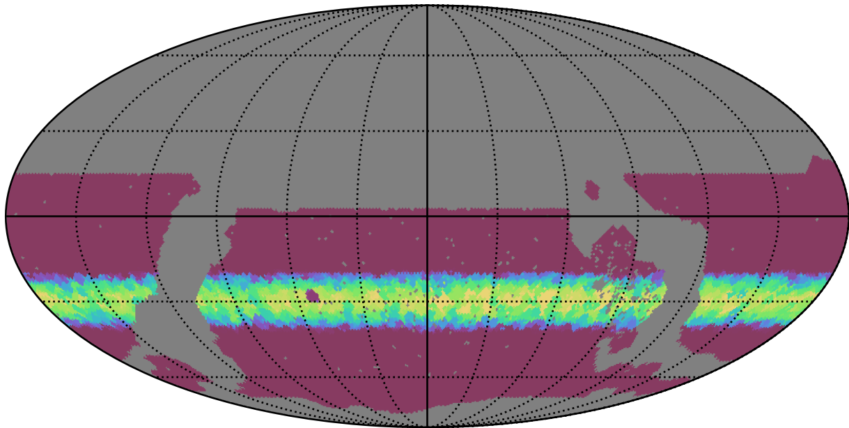
noroll_mjdp0_v3.4_10yrs WFD all bands: Min normairmass
