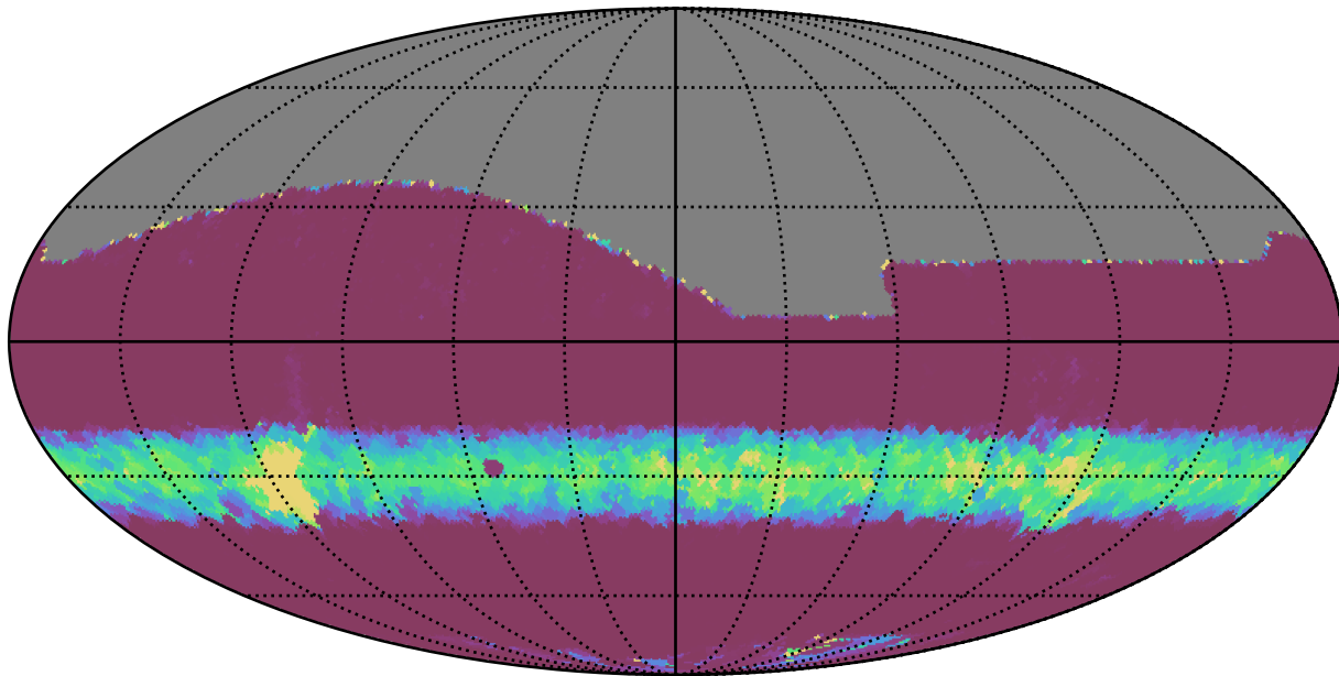
noroll_mjdp0_v3.4_10yrs All sky z band: Min normairmass
