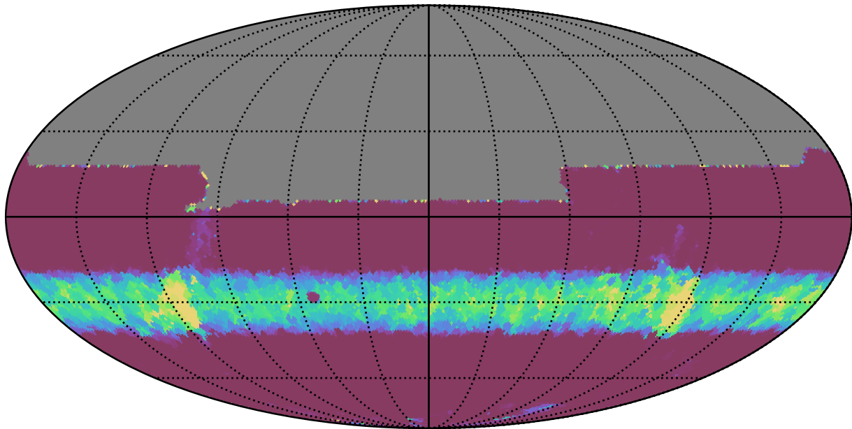
noroll_mjdp0_v3.4_10yrs All sky y band: Min normairmass
