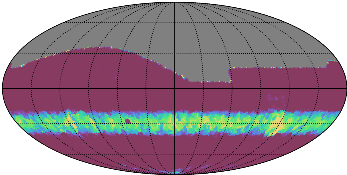
noroll_mjdp0_v3.4_10yrs All sky r band: Min normairmass
