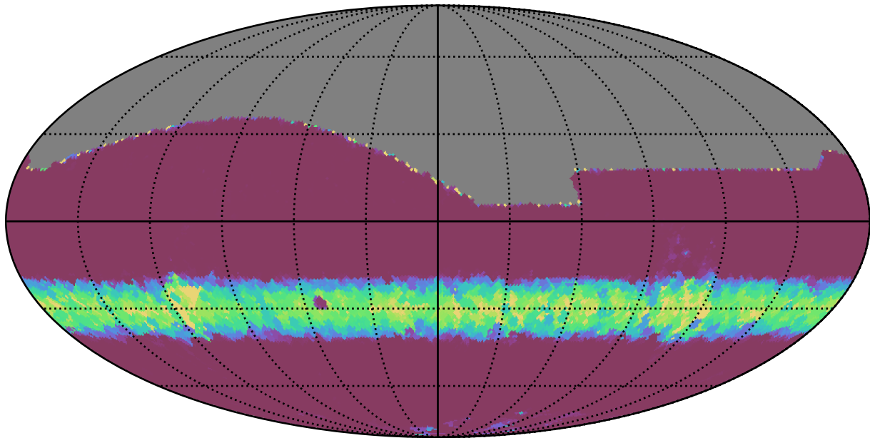
noroll_mjdp0_v3.4_10yrs All sky i band: Min normairmass
