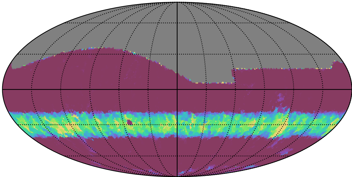
noroll_mjdp0_v3.4_10yrs All sky g band: Min normairmass
