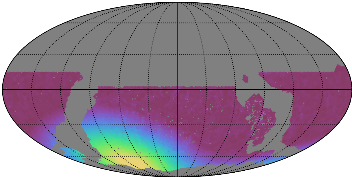
noroll_mjdp0_v3.4_10yrs WFD z band: Min moonDistance
