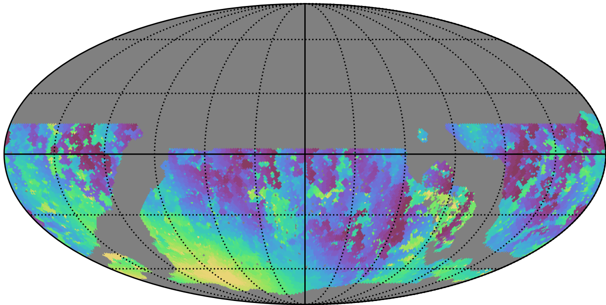
noroll_mjdp0_v3.4_10yrs WFD u band: Min moonDistance
