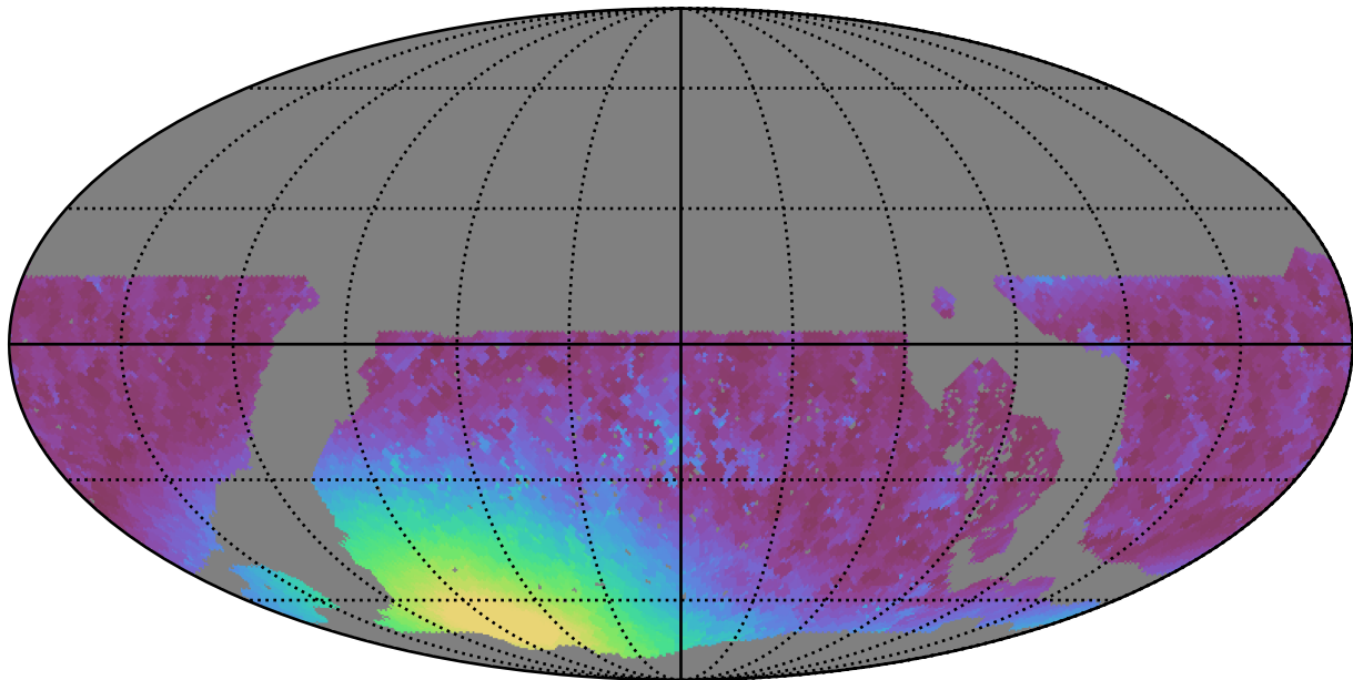
noroll_mjdp0_v3.4_10yrs WFD r band: Min moonDistance
