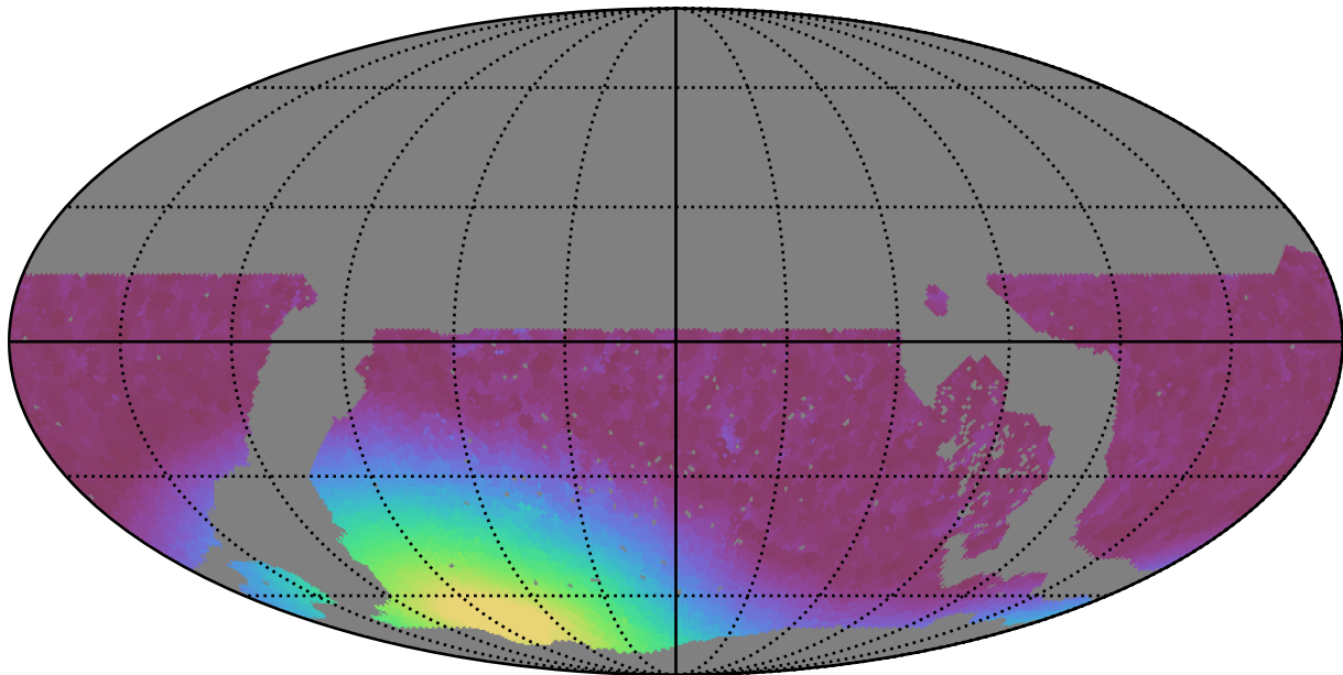
noroll_mjdp0_v3.4_10yrs WFD i band: Min moonDistance
