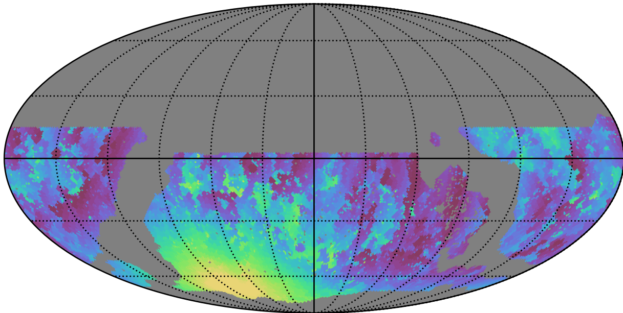
noroll_mjdp0_v3.4_10yrs WFD g band: Min moonDistance
