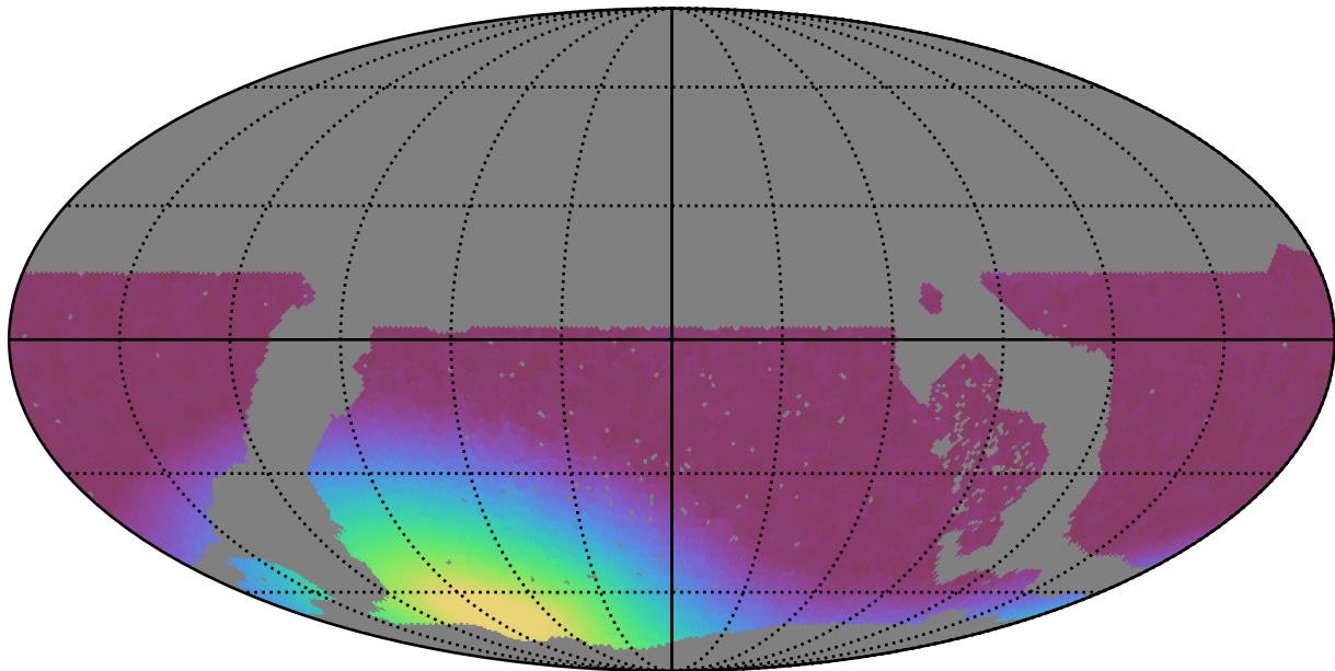
noroll_mjdp0_v3.4_10yrs WFD all bands: Min moonDistance
