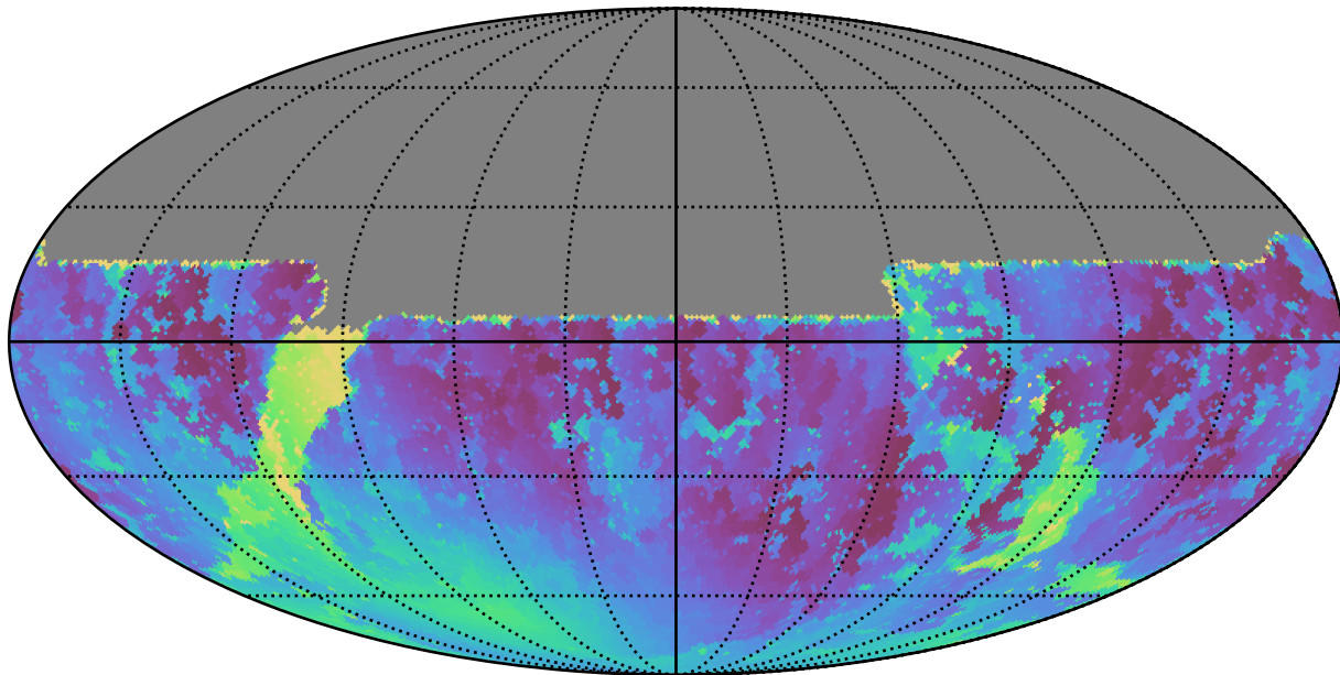
noroll_mjdp0_v3.4_10yrs All sky u band: Min moonDistance
