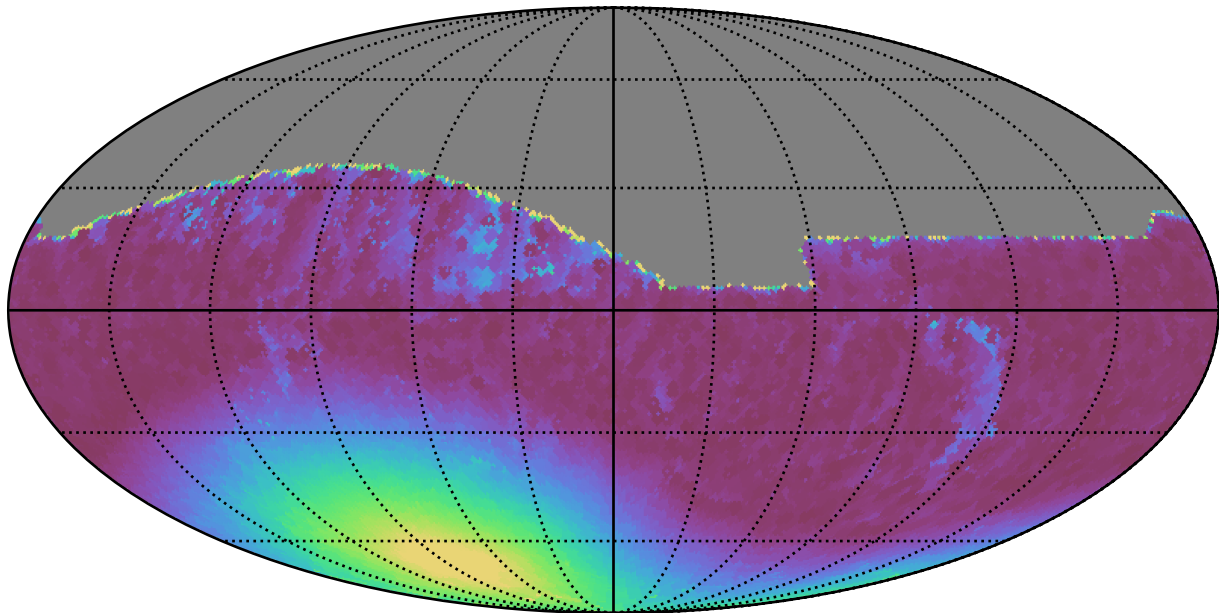
noroll_mjdp0_v3.4_10yrs All sky i band: Min moonDistance
