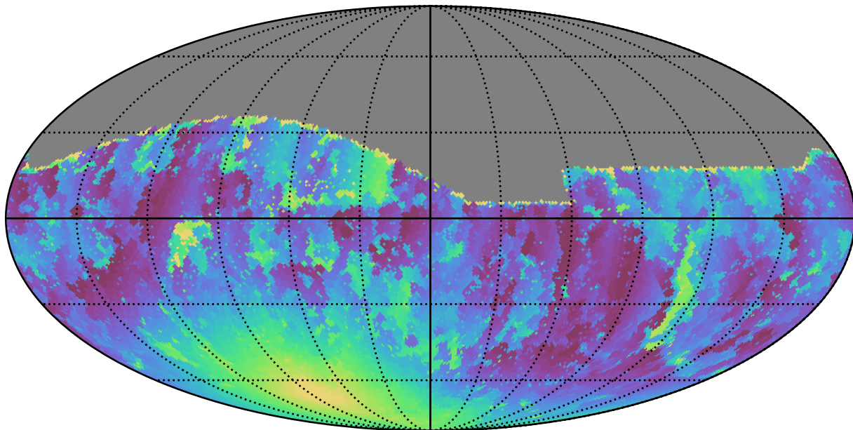
noroll_mjdp0_v3.4_10yrs All sky g band: Min moonDistance
