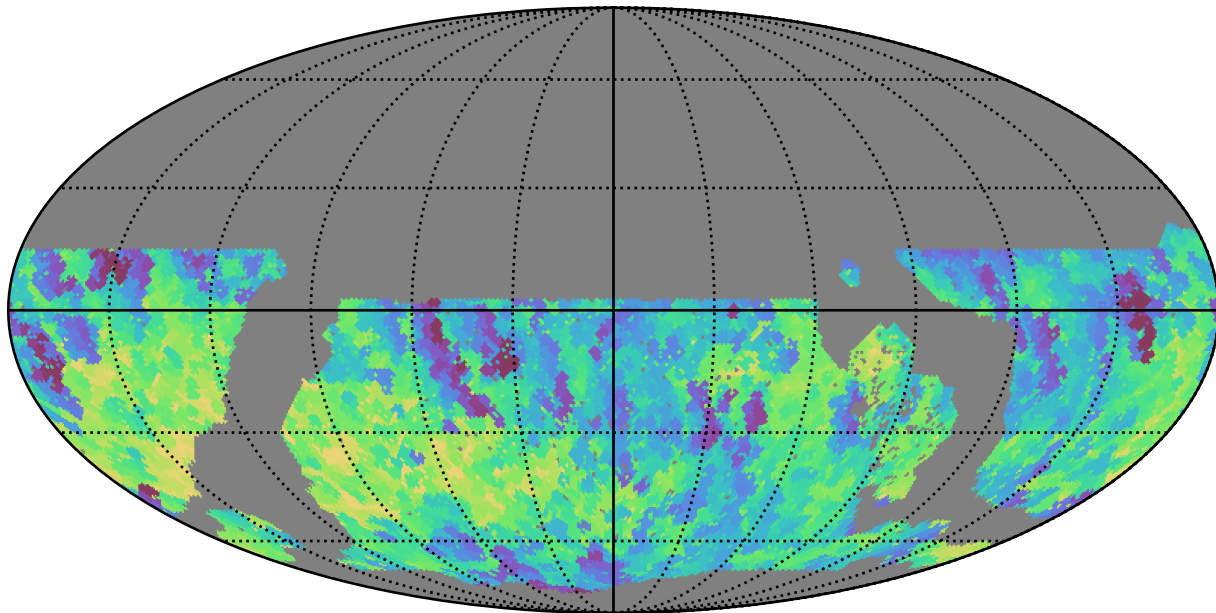
noroll_mjdp0_v3.4_10yrs WFD all bands: Min fiveSigmaDepth
